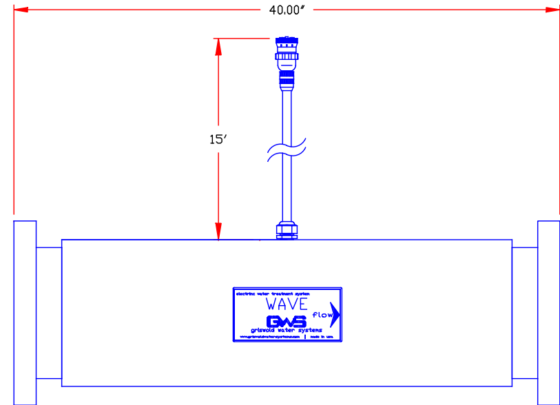
8" FLG. FRP RC ELEVATION SCH 40 PVC SHELL
