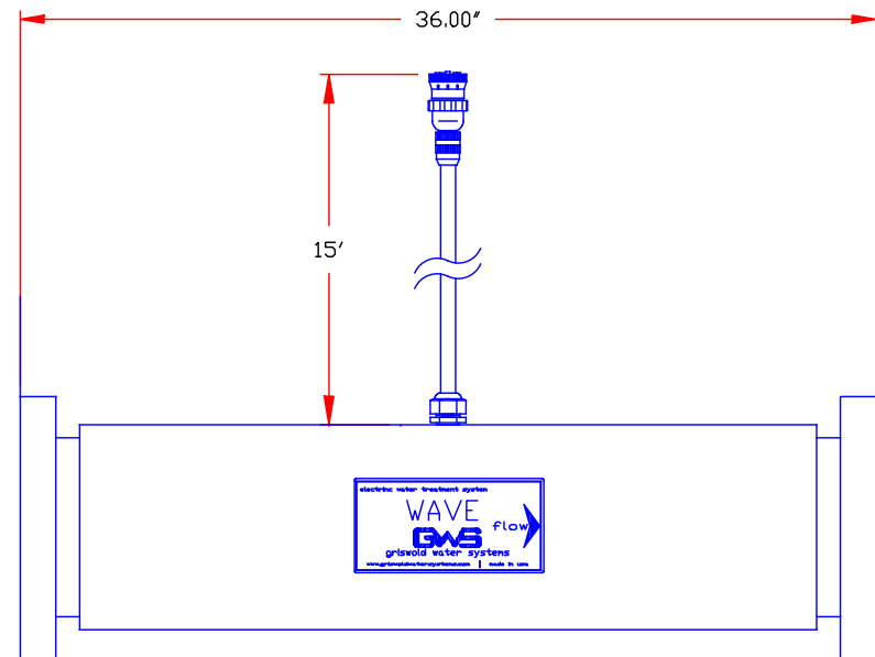
6" FLG. FRP RC ELEVATION SCH 40 PVC SHELL
