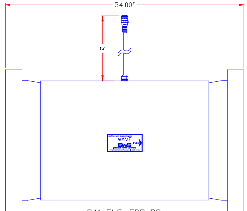
24" FLG. FRP RC ELEVATION SCH 40 PVC SHELL
