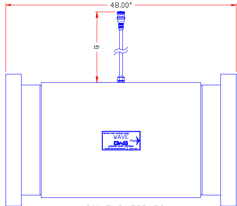
20" FLG. FRP RC ELEVATION SCH 40 PVC SHELL
