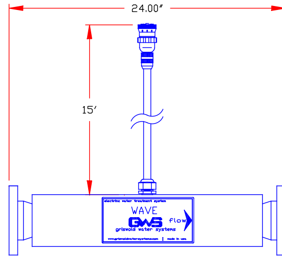
2" FLG. FRP RC ELEVATION SCH 40 PVC SHELL
