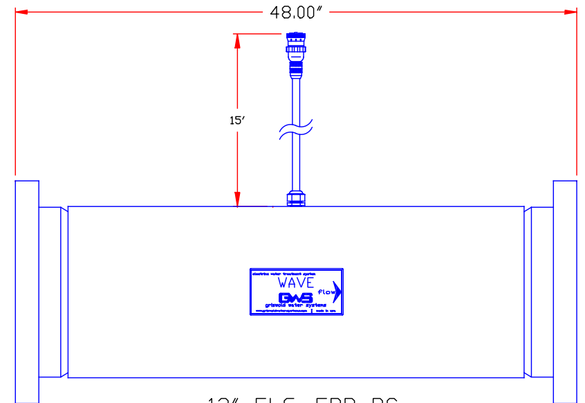
12" FLG. FRP RC ELEVATION SCH 40 PVC SHELL
