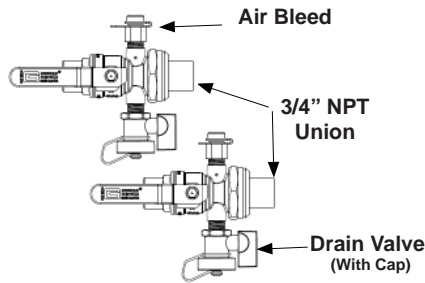
VALVE PACKAGE (VP-75)
