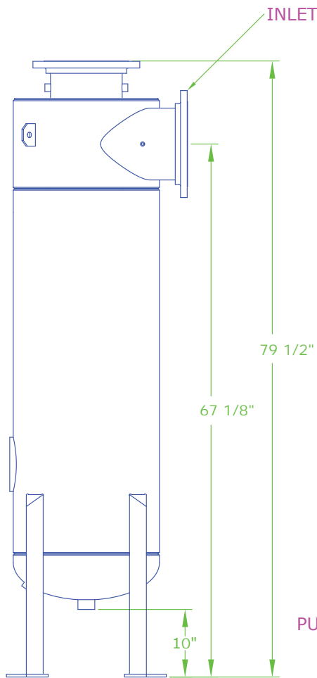
ELEVATION VIEW
