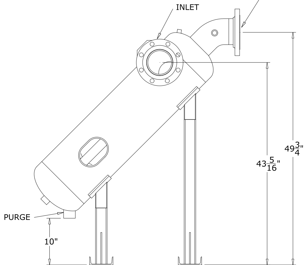
ELEVATION VIEW
